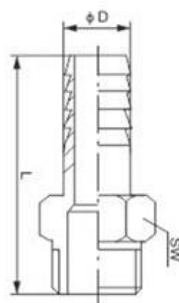
201/304 Hex hose nipple 201/304
