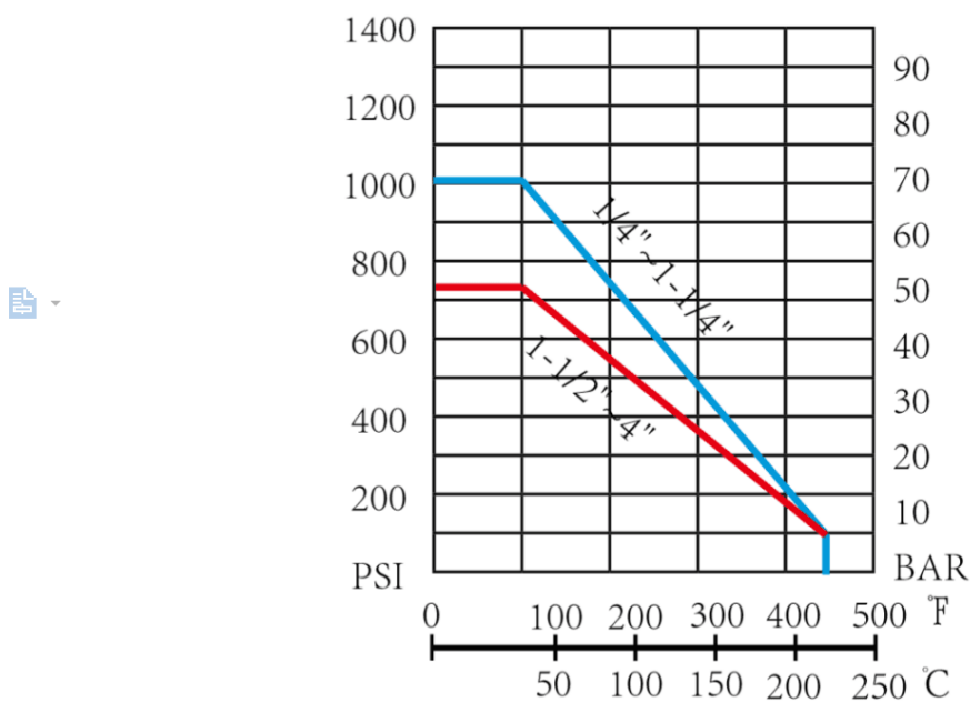
Pressure-Temperature Rating 1/4"~4"
