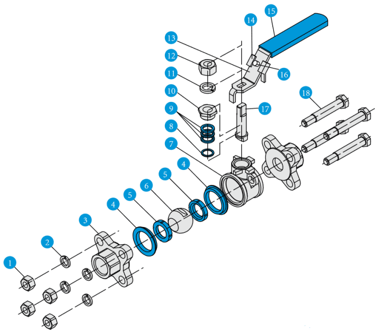
PART DRAWING
